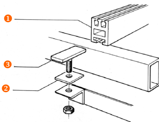
Fixing of channel section on screen crossbeam SP
