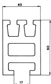
Light alloy channel section SP
